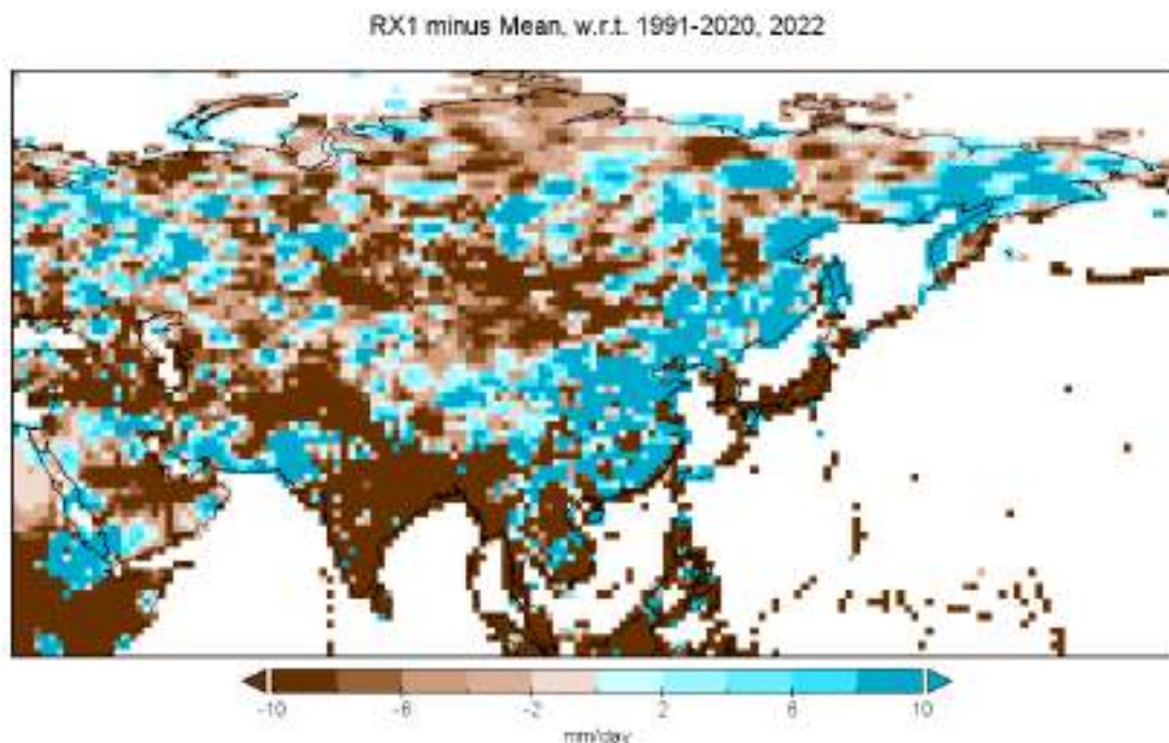
Figure 6. Difference between the highest daily precipitation totals in 2022 and the 1991–2020 long-term mean. Blue indicates the regions with more extreme daily precipitation than the long-term mean. Brown indicates the regions with less extreme daily precipitation than the long-term mean. Source: GPCC, Deutscher Wetterdienst, Germany
