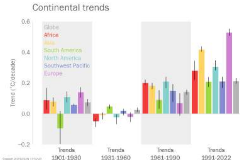
Figure 4. Trends in mean surface air temperature for the six WMO regions and the global mean (°C) over four sub-periods using the six data sets. The bars indicate the trend in the mean of the data sets. The black lines indicate the range between the largest and the smallest trends in the individual data sets.
