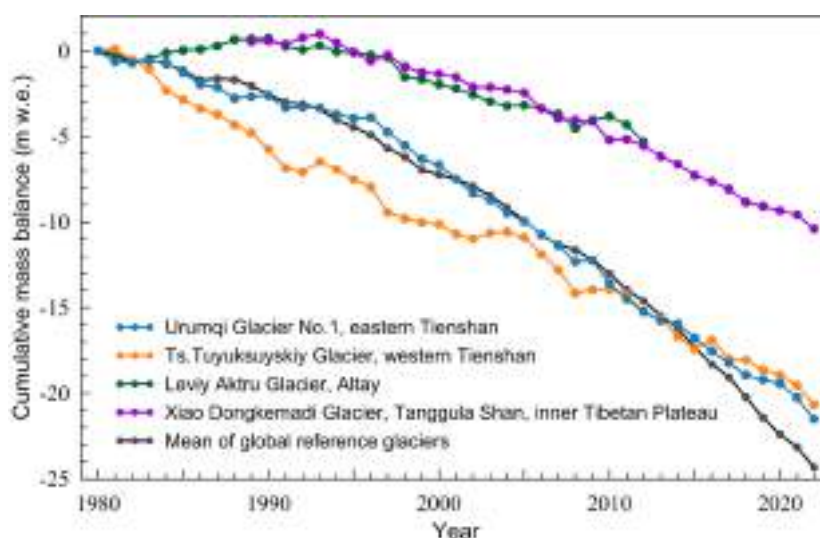
Figure 7. Cumulative mass balance (in metres water equivalent (m w.e.)) of four reference glaciers in the High Mountain Asia region and the average mass balance for the global reference glaciers
