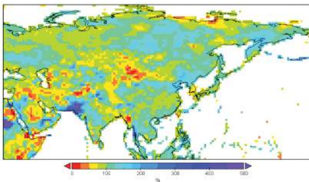
Figure 5. Precipitation anomalies for 2022, expressed as a percentage of the 1991–2020 average Source: Global Precipitation Climatology Centre (GPCP), Deutscher Wetterdienst, Germany
